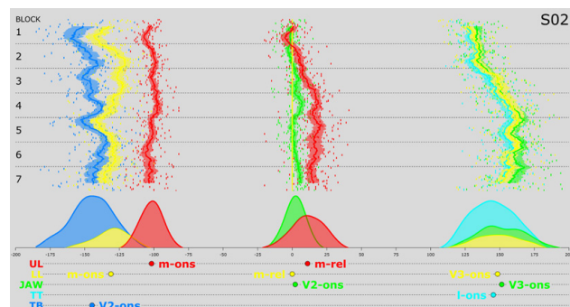
Figure 2: Articulatory landmarks and moving-averages with \pm 2 s.e. (50-trial window) for speaker S02. Landmarks are aligned to LL [m] release.
