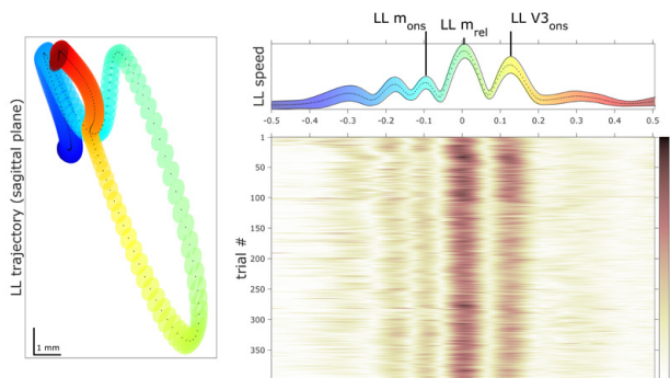
Figure 1: Example of aligned speed time series from participant S01, with LL trajectory (left), mean LL speed trajectory \pm 1 s.d. (upper right), and LL speed trajectories aligned across trials (lower right).
